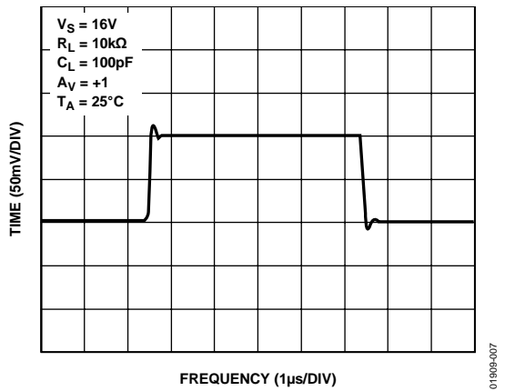
Figure 7. Small Signal Transient Response
