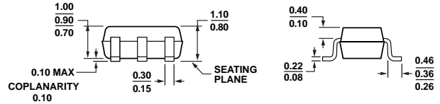
Figure 35. 5-Lead Thin Shrink Small Outline Transistor Package [SC70] (KS-5) Dimensions shown in millimeters
