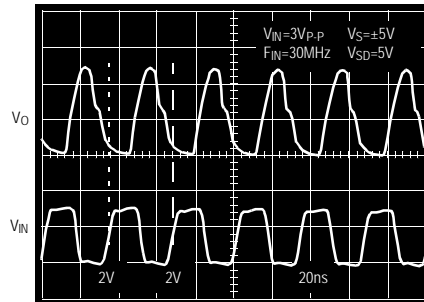
Output with 30MHz Input VIN=3Vp-p
