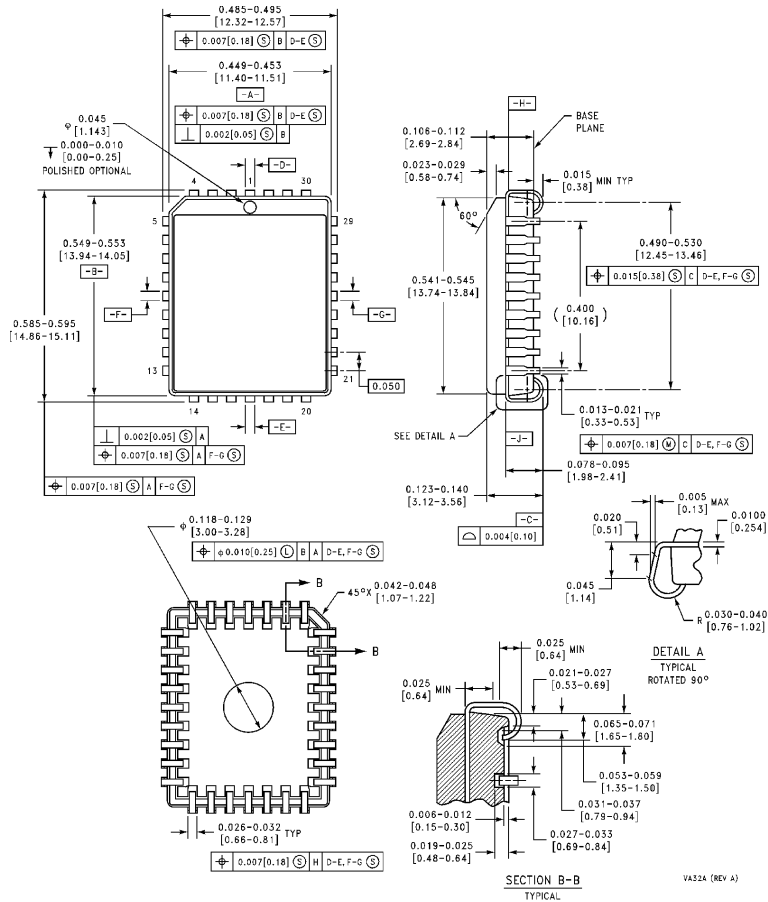
32-Lead PLCC Package (V) Order Number NM27LV010BVXXX Package Number VA32A
